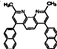
Structural formula 10:
